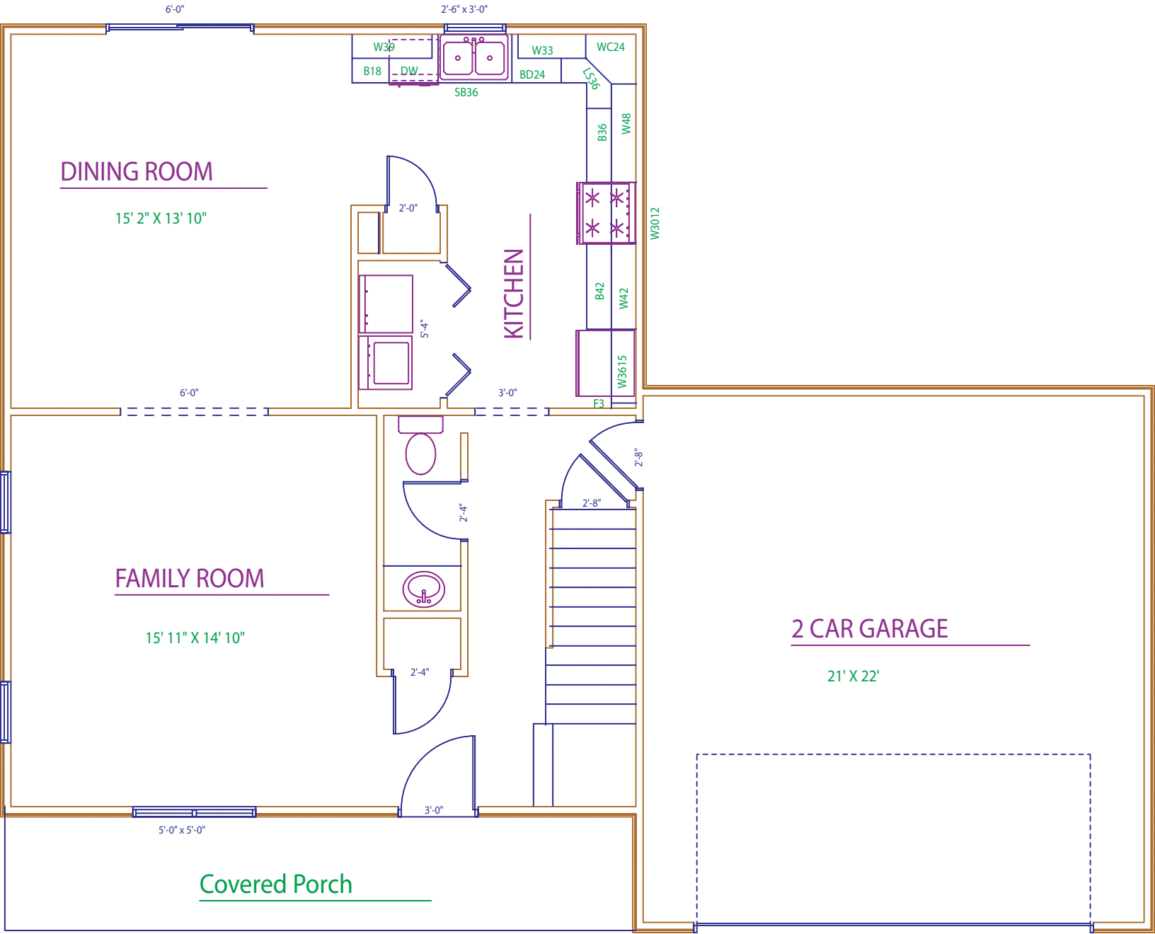
JOSHUA TREE First Floor Plan
